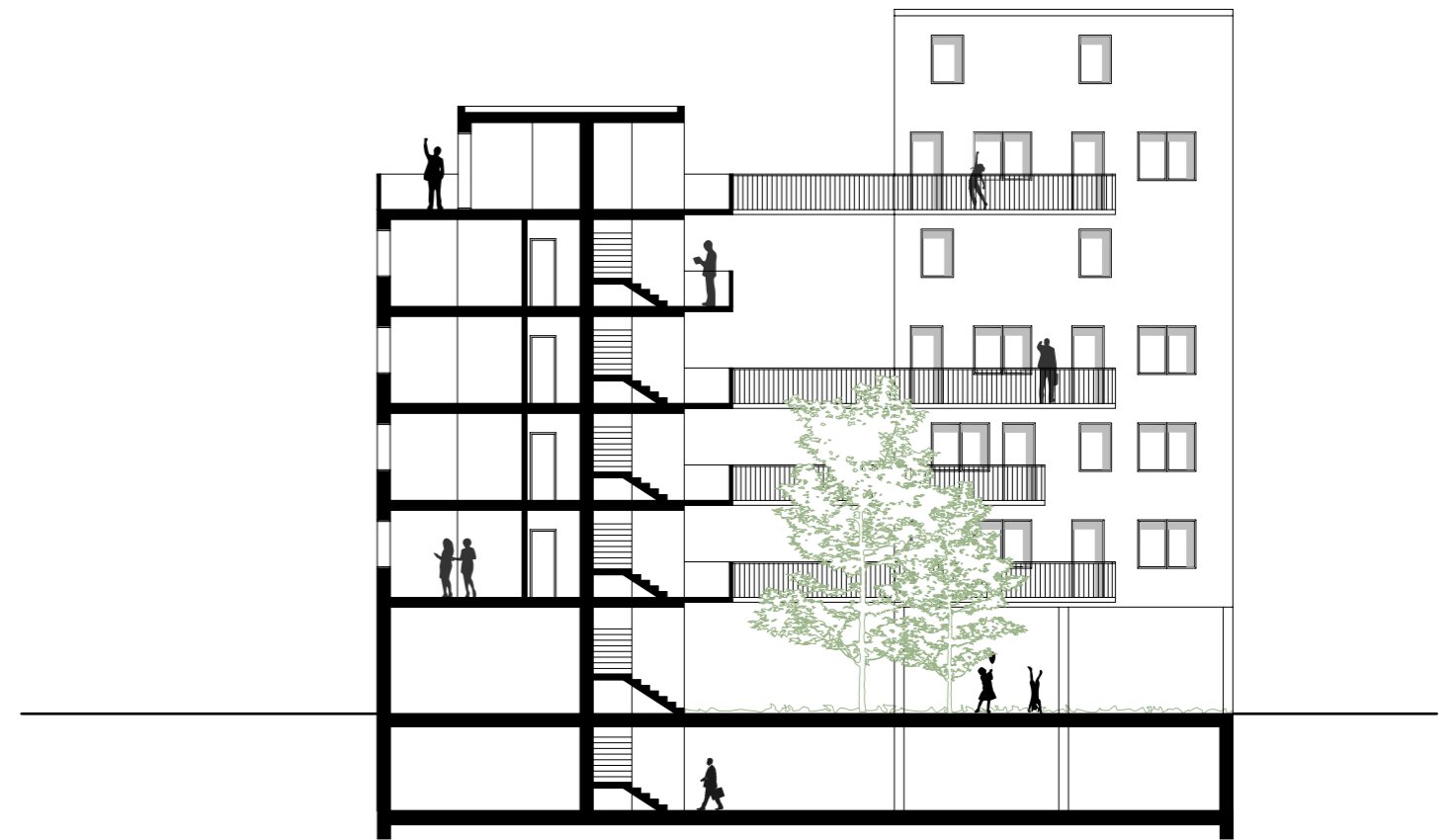
SECTION B-B'
